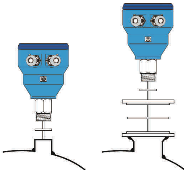
Figure 1. Mounting
