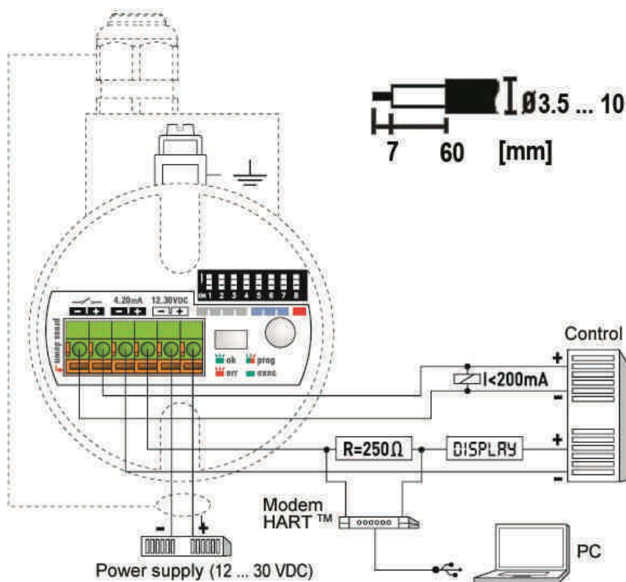
Figure 3. Electrical connection
