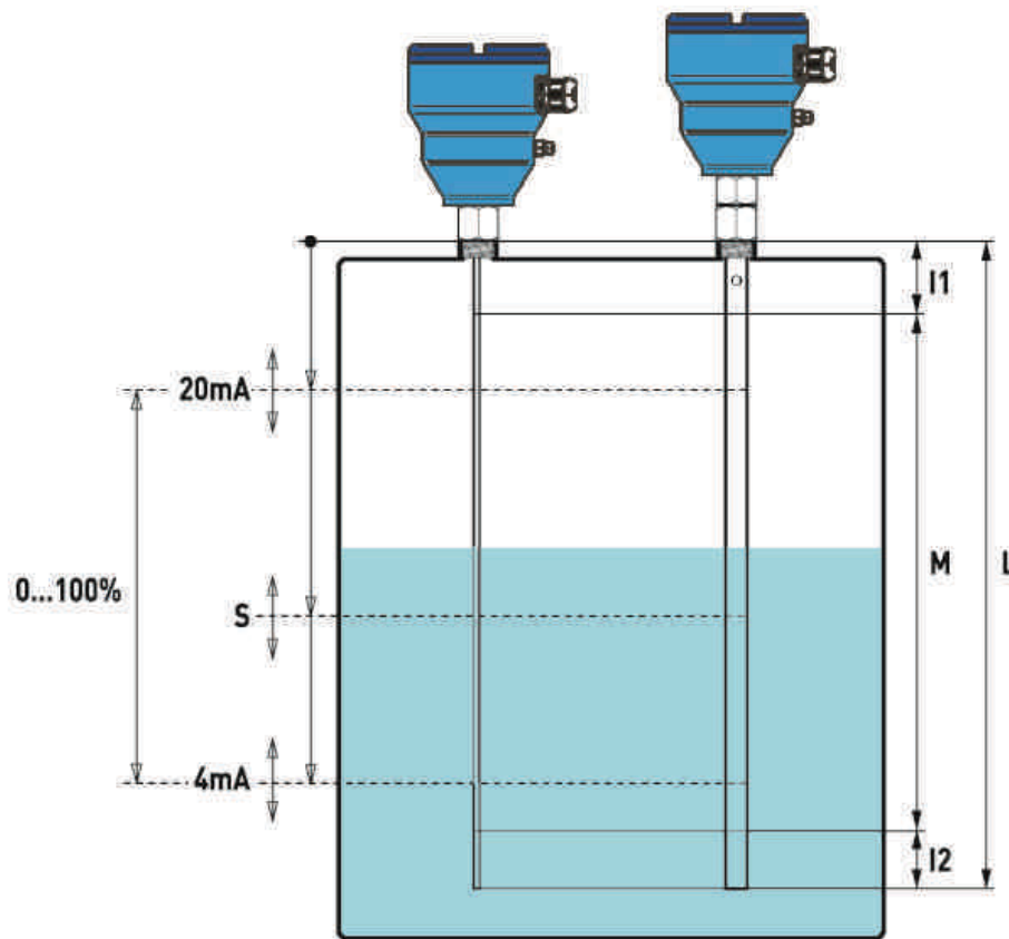
Figure 10. Probe length and measuring range
