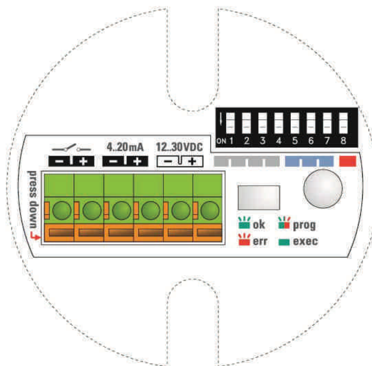
Figure 4. Control elements
