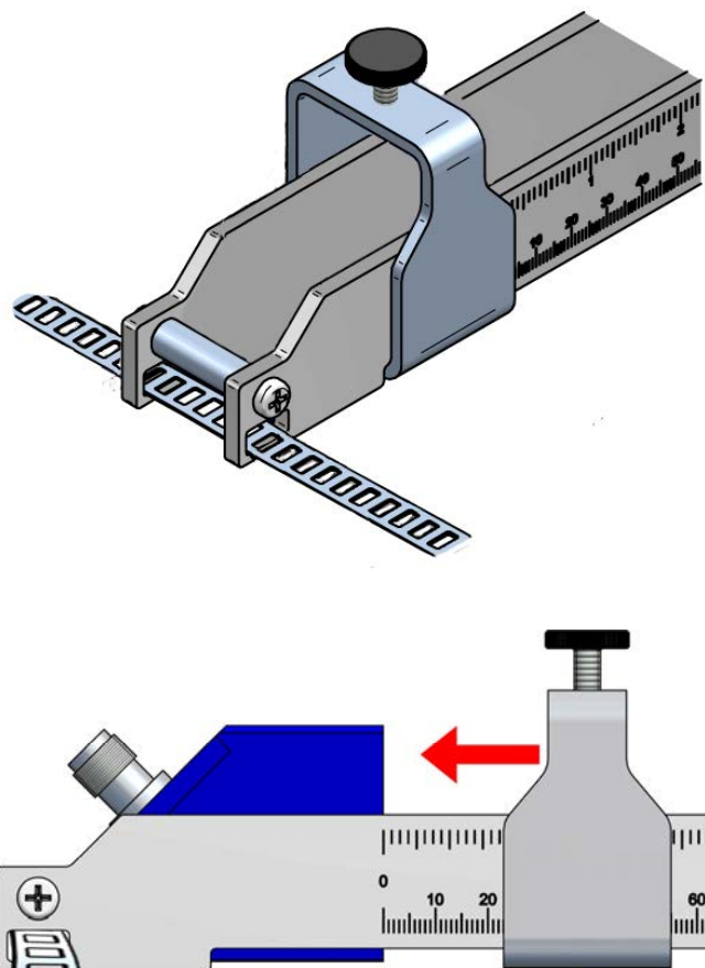
Fig. 4. Guide and guide strap DN80 ... DN350
