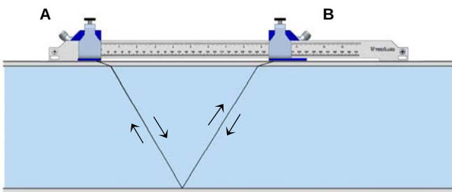
Fig. 1. V-type installation (DN ≤ DN350)
